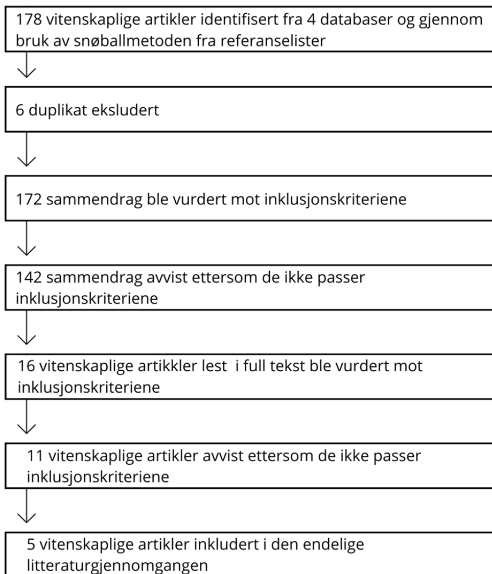
Figur 3: PRISMA- diagram
