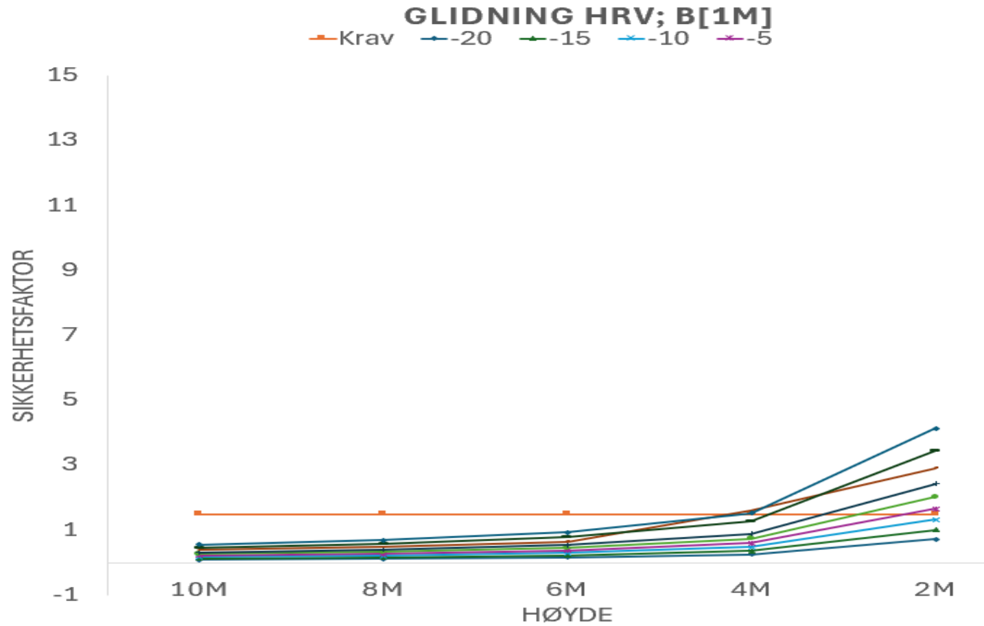
Figur 1 TT, Glidning HRV [1m] islast[0kN/m]
