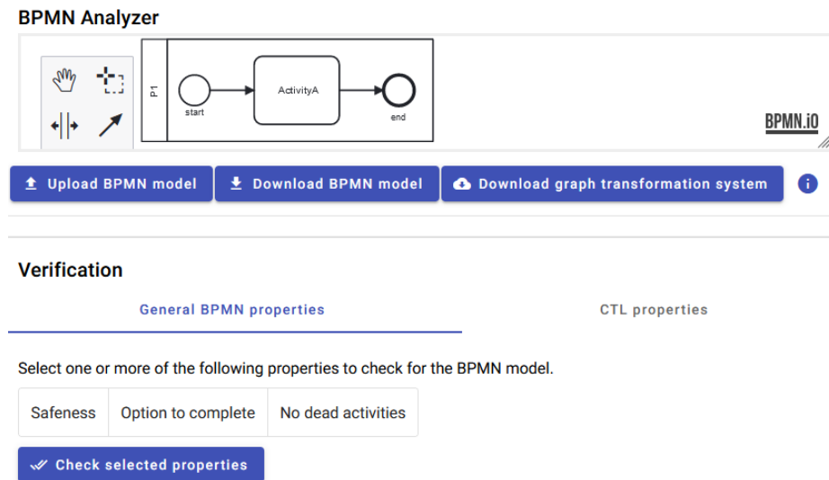
Fig. 15. Screenshot of the BPMN Analyzer tool
