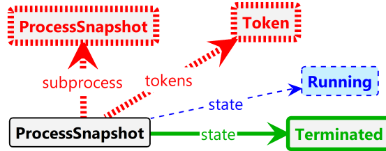
Fig. 9. Termination rule in Groove
