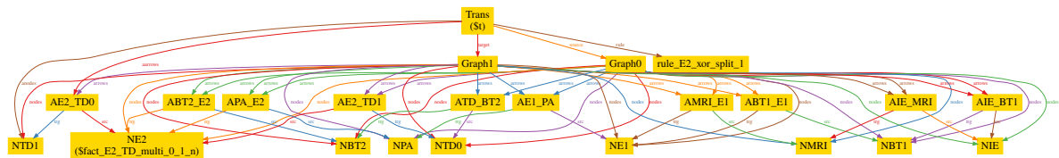
Figure 3: Counterexample of xor_split
