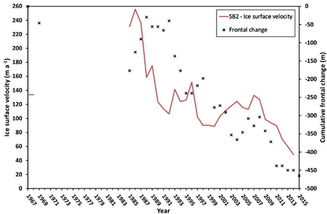
Fig. 6. Cumulative frontal change of Glaciar Universidad, between 1967 and 2015, compared with ice surface velocity fluctuations measured for SB2 (location shown in Fig. 1). Y-axis point labels for frontal change represent second year of observation period (e.g. 2015 = frontal change between 2014 and 2015). Y-axis point labels for ice surface velocity are the same as stated in Figure 3.
