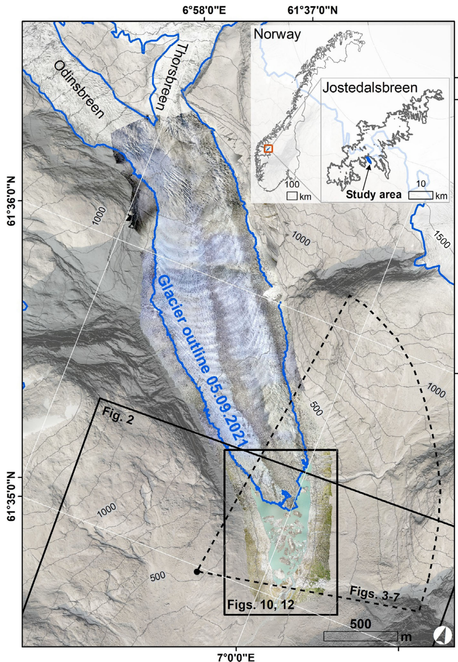
FIGURE 1 Location map of the study area, the lower part of Austerdalsbreen. The blue outline shows the glacier outline in September 2021 and the orthophotomosaic shows results from a UAV-based survey during 3–5 September 2021. The dashed line approximately shows the area covered by annual terrestrial photography since 1991 (approximate photographer's position: black dot). [Colour figure can be viewed at wileyonlinelibrary.com ]
