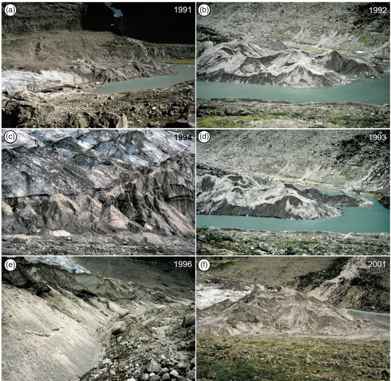
FIGURE 4 Morphological processes at the terminus of Austerdalsbreen during the recent advance in the 1990s: (a) Active lower glacier tongue (right) and static down-valley complex of stagnant ice and debris (left), 31.08.1991; (b) Debris-ice complex on 11.08.1992; (c) Prominent shear planes and ice-scree fans along the latero-frontal margin, 08.08.1994; (d) Debris-ice complex on 12.08.1993—note the development of ice-disintegration features and local expansion of a glacial pond in comparison to (b); (e) Ice overriding remnants of ice-scree fans and (subsequently) older latero-frontal moraines, 21.08.1996; and (f) View of the frontal glacier margin showing the final stage of development of the former debris-ice complex when the advance ceased, 29.08.2001 (note that photos (c) and (e) are taken from lower positions slightly up-glacier. Photographs: Stefan Winkler. [Colour figure can be viewed at wileyonlinelibrary.com ]
