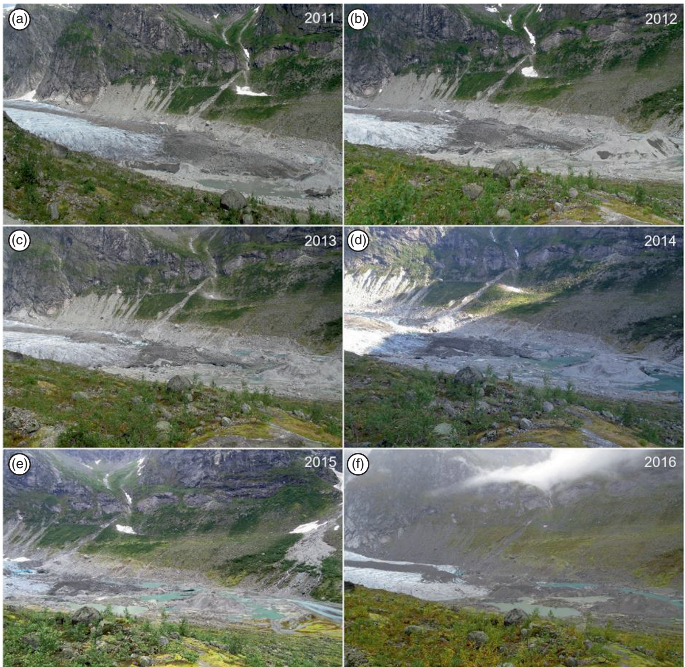
FIGURE 6 Degradation of the glacier front of Austerdalsbreen 2011–2016: (a) 28.07.2011; (b) 08.08.2012; (c) 29.08.2013; (d) 09.08.2014; (e) 17.09.2015; and (f) 24.09.2016. The first signs of formation of a new glacial lake started to show during this period. In 2014–2015, the frontal ice-cored moraine was detached from the active glacier ice. Photographs: (d) Per Solnes, all other photographs by Jacob C. Yde. [Colour figure can be viewed at wileyonlinelibrary.com ]
