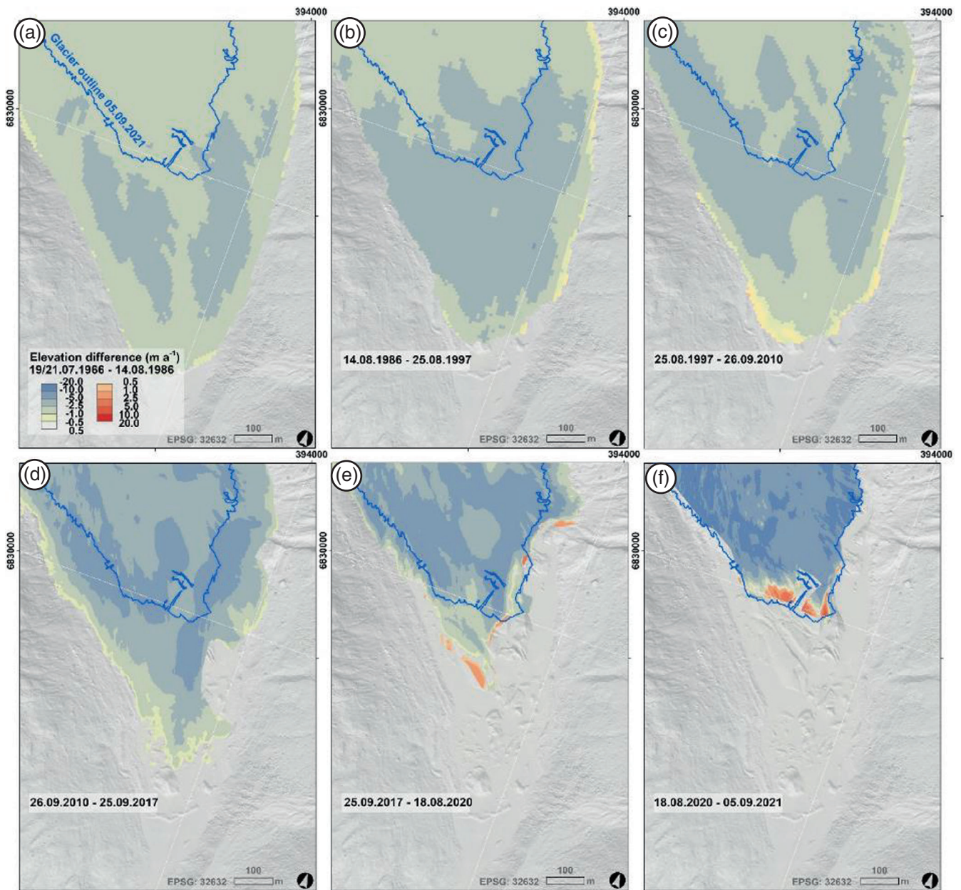
FIGURE 10 Map showing elevation differences and front recession throughout the observation period at the terminus of Austerdalsbreen. [Colour figure can be viewed at wileyonlinelibrary.com ]
