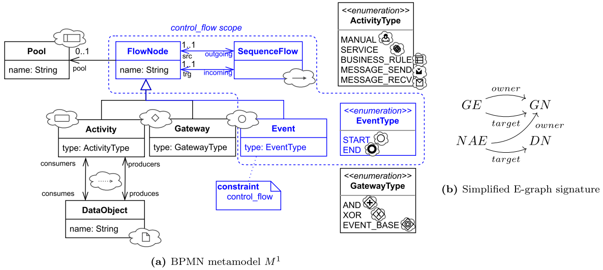
Fig. 6. Metamodel Example and Base Language Signature
