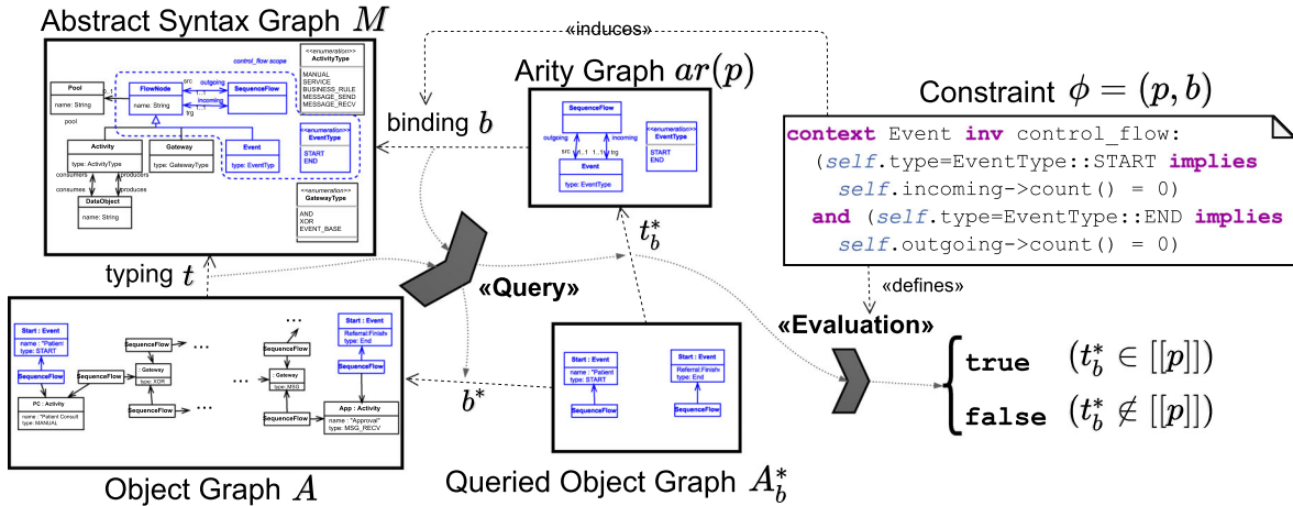
Fig. 7. Diagrammatic Constraints in a Nutshell
