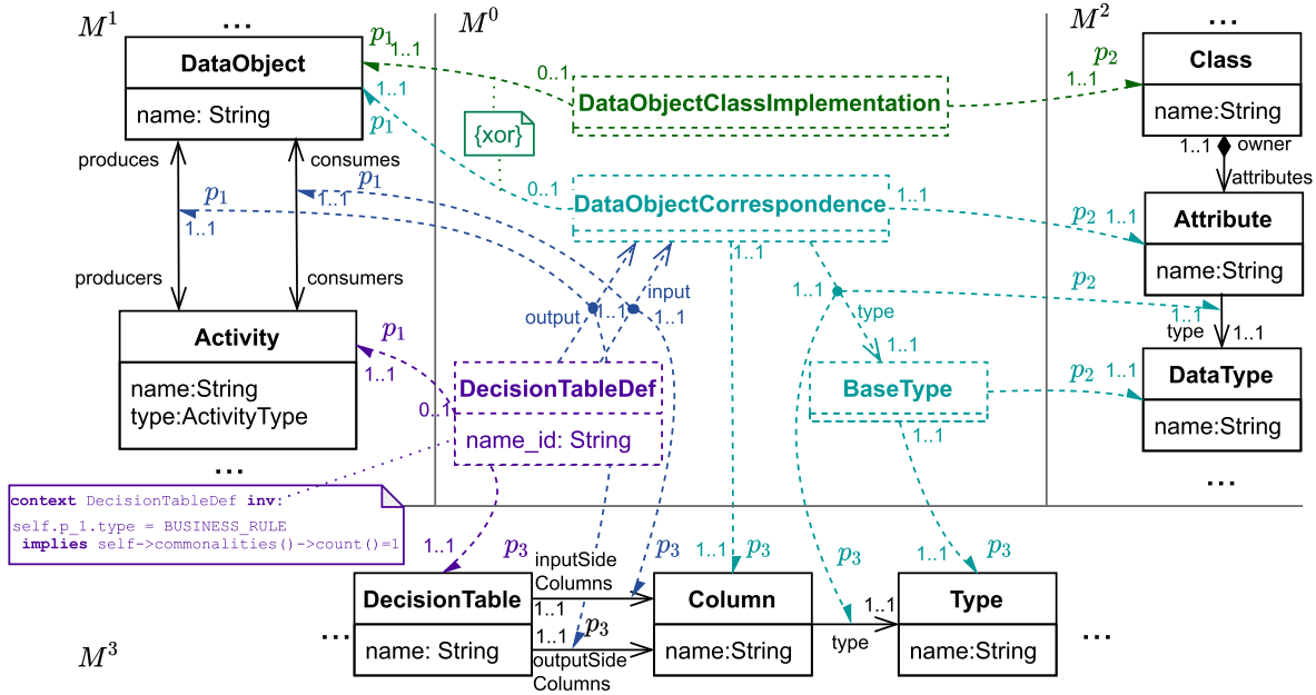
Fig. 8. Commonality representative metamodel M^0
