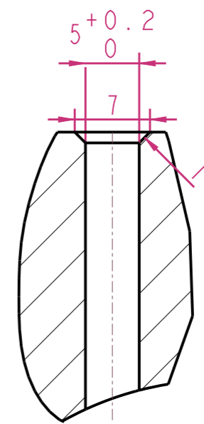
DETAIL A SCALE 2:1
