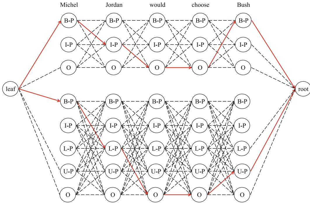
Fig. 5. The proposed latent variable CRF I (LVCRF-I).
