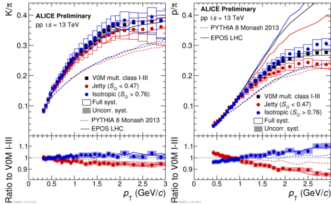
Fig. 3. Top panels: p_T -differential K/\pi and p/\pi ratios in VOM multiplicity class I–III events, jetty events (20% lowest S_0 ) and isotropic events (20% highest S_0 ). Bottom panels: p_T -differential K/\pi and p/\pi double-ratios in jetty and isotropic events to VOM class I–III events. Results are compared with PYTHIA 8 and EPOS LHC models.
