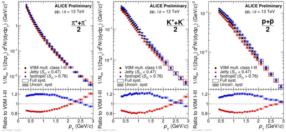
Fig. 2. Top panels: transverse momentum spectra of \pi^\pm , K^\pm , and p(\bar{p}) in VOM multiplicity class I–III events, jetty events (20% lowest S_O ) and isotropic events (20% highest S_O ). Bottom panels: ratio of spectra in jetty (isotropic) events to the VOM class I–III.
