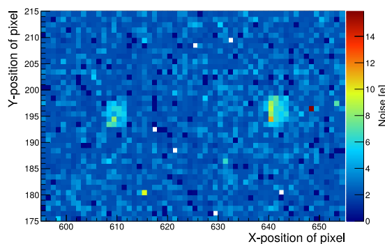
Fig. 4. Noise map of ALPIDE chip zoomed in on the two positions irradiated with ^4\text{He} ion beam. The noise at these two positions may have increased due to the received dose. The dose delivered to the left spot is about 1.3 kGy and to the right is about 13 kGy. This dose is roughly equivalent to the 1 M pCT scan and 10 M pCT scans, respectively.
