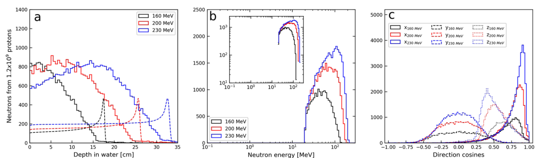
Figure 3. Characteristics of the detected neutrons produced in the water phantom for the 160, 200 and 230 MeV proton beams as obtained from MC simulations. (a) Production depth distributions for detected neutrons. Relative depth doses are shown with dashed lines (arbitrary dose units). (b) Distribution of initial kinetic energy of detected neutrons. The neutron spectra are shown both with linear (main plot) and logarithmic (inlay) ordinate axis. The absence of data below 20 MeV is due to the exclusion of low energy neutron scattering events ( E_n < 20 MeV) in the reconstruction of neutron production distributions. (c) The initial angular distribution of detected neutrons. Direction cosines are shown for the direction along the beam axis (x, solid histogram) and the y- and z-axes (dashed and dotted histograms), perpendicular to the initial beam direction.
